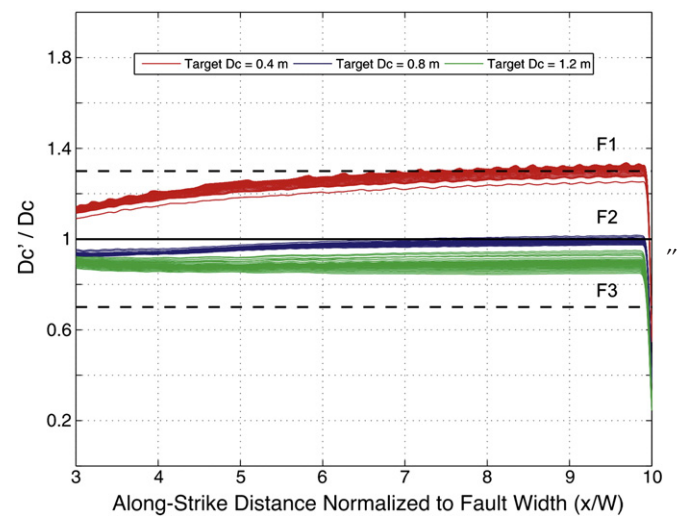
Fig. 3. Estimates of D_c^*/D_c ratios for rupture cases F1 (red curves, D_c = 0.4 m), F2 (blue curves, D_c = 0.8 m) and F3 (green curves, D_c = 1.2 m) estimated along strike-parallel profiles on the fault from the earth surface to a depth of 0.7W .
