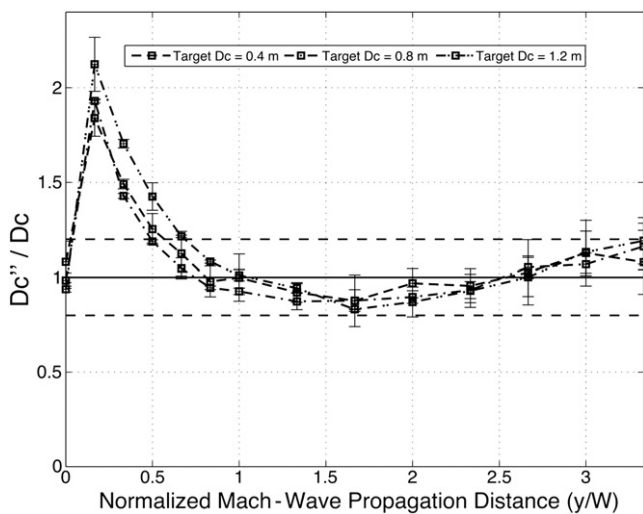
Fig. 11. Average ratios of D_c^e/D_c along receiver lines L1, L2 and L3 for cases F1–F3. The error bars depict the mean \pm 1 standard deviation, and the dashed lines represent deviations of 20% from a perfect fit between D_c^e and D_c .
